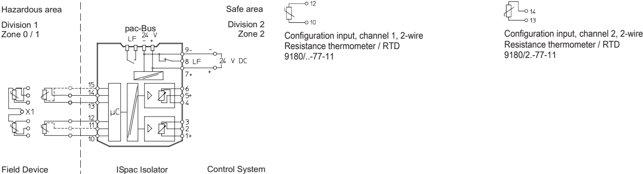
Connection diagram 9180/2.-77-11
