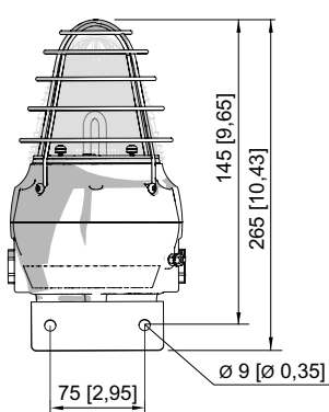
FX15 Beacon with L-bracket
