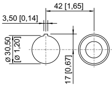
Drilling pattern: for aligning several devices Ø 38 mm, in a panel
