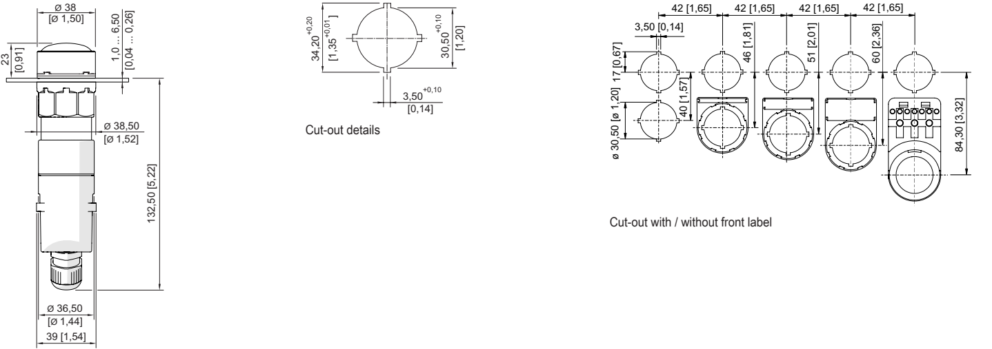
8013/3.1, 8013/3.3 Indicating lamp with terminal compartment
