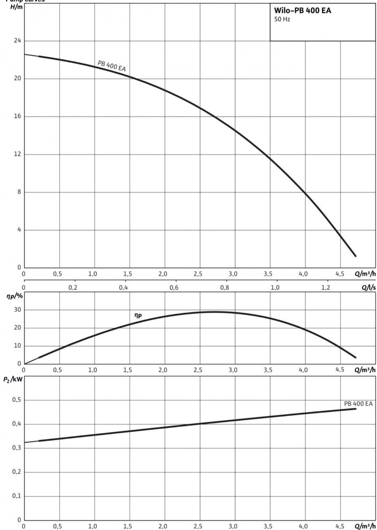
Pump curves
