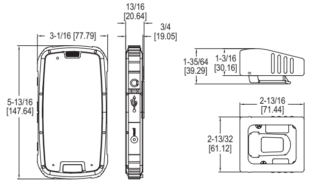
UHH-BTG Wireless Mobile Gateway
