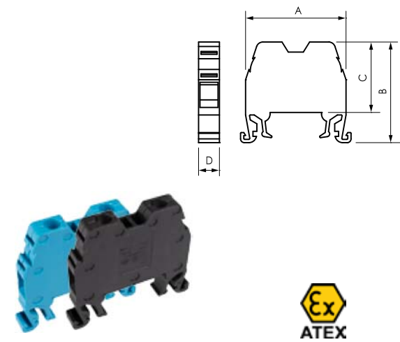
Neutral terminals. Screw connection
