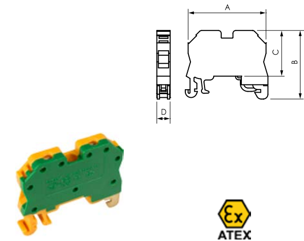
Earth terminal connection. Screw connection
